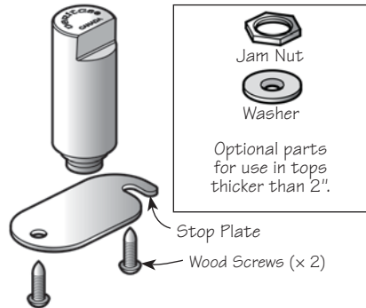
Figure 1: Prairie dog parts.
