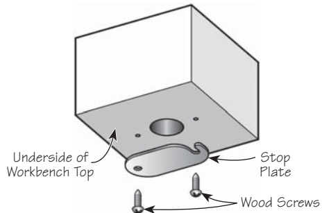
Figure 3: Plate installation.
